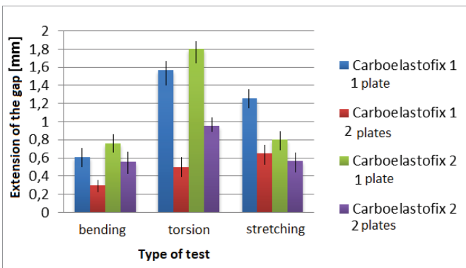
Figure 5: The expansion of fissure in particular types of fatigue tests.
