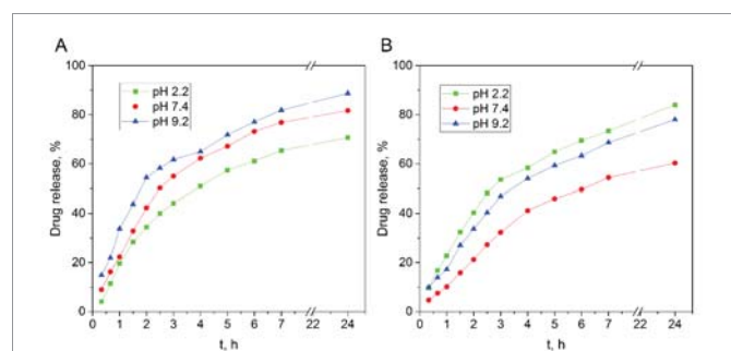
Figure 4: Effect of time on in-vitro drug release profiles of QTG-AA A. QTG-AM. B. Hydrogels in PBS at different pHs.
