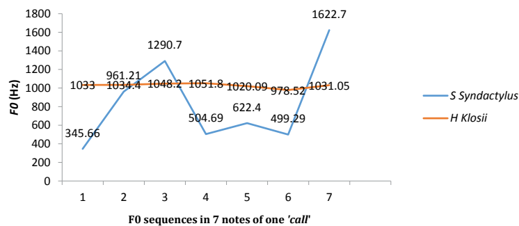
Figure 3: The call 'call' dynamics of F0 between S.syndactylus and H.klosii show that the S.syndactylus pitch pattern is more dynamic that begins with a low tone at the beginning and then rises in the pre-trill and first trill, down on the second trill, slightly up on the third trill, and back down on the fourth trill, back up with the highest tone on the fifth trill. While the tone pattern (pitch) H.klosii tend to be more monotonous or flat.
