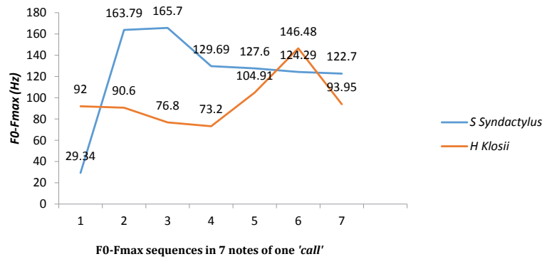
Figure 4: The 'call' dynamics in F0-Fmax between S.syndactylus and H.klosii show that the sound of the S.syndactylus vowel resonates maximally in the pre-trill and the first trill while the H.klosii vocal sound resonates maximally on the sixth trill.
