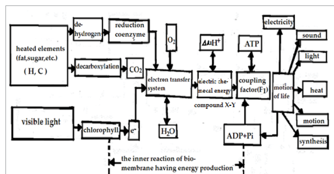
Figure 3: The energy current of life-matters [4], where ΔμH + is difference of electric-chemical potential of H + [3,6-8]. Walker shared the 1997 Nobel Prize in chemistry.
