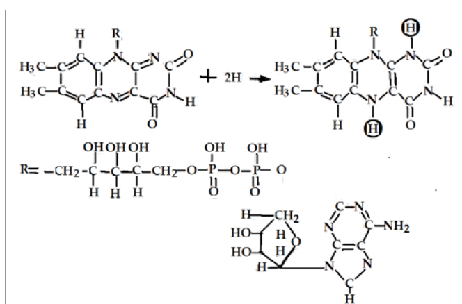
Figure 2: The reaction of generation of reduced type (FAD-H 2 ) from reffavin adenine dinucleotide (FAD) through capturing hydrogen atom [3,6-8].
