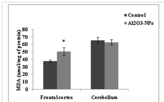
Figure 4: Effect of Al 2 O 3 -NPs injections on MDA levels in FC and Cb. Values are given as mean ± SEM. (*) significant mean Al 2 O 3 -NPs treatment effect (p ≤ 0.05).
