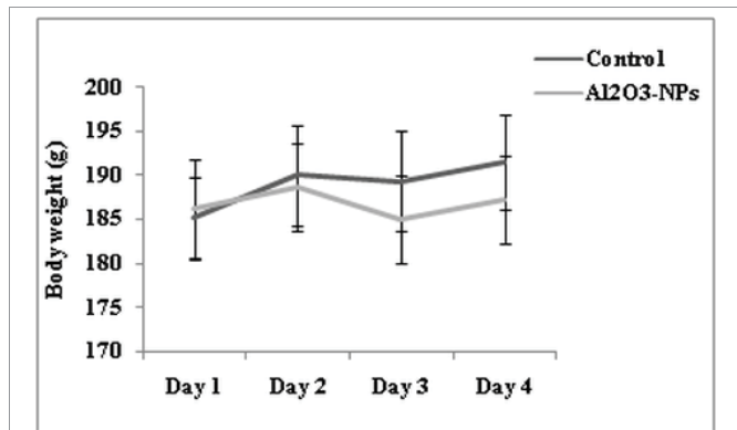
Figure 3: Body weight changes for rats treated with Al 2 O 3 -NPs. Values are given as mean ± SEM of 12 animals per group.
